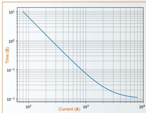
Model NH00-80A
