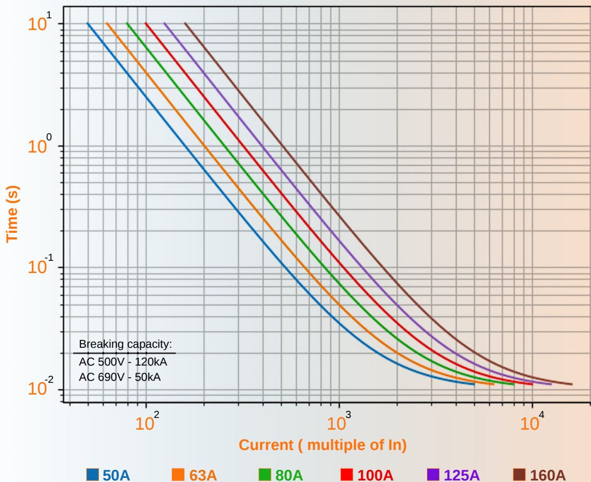
Type gG Fuse Time-Current Characteristic (IEC 60269 - Illustrative)
