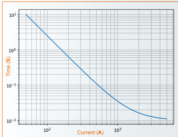
Model NH00-50A
